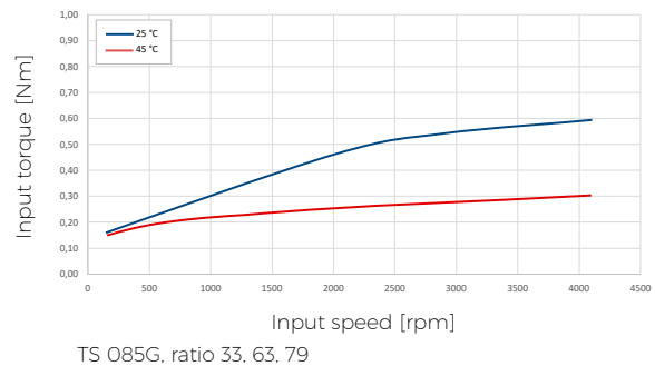
Fig. 3.15: No-load running torque charts
