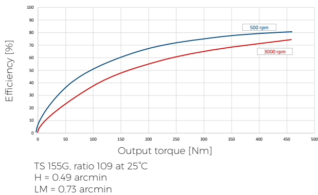
Fig. 3.13: Efficiency charts
