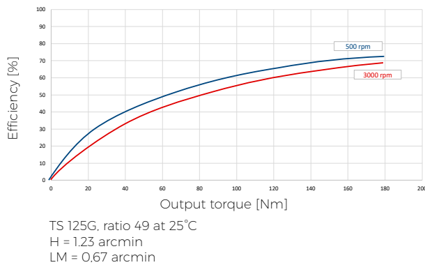
Fig. 3.14: Efficiency charts
