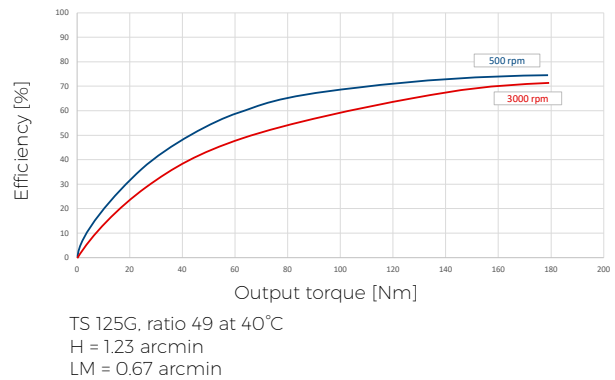
Fig. 3.14: Efficiency charts
